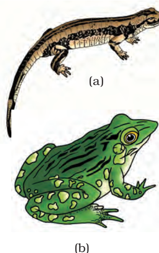
Figure 4.21 Examples of Amphibia : (a) Salamandra (b) Rana
