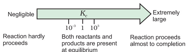
Fig. 7.6 Dependence of extent of reaction on K_c
