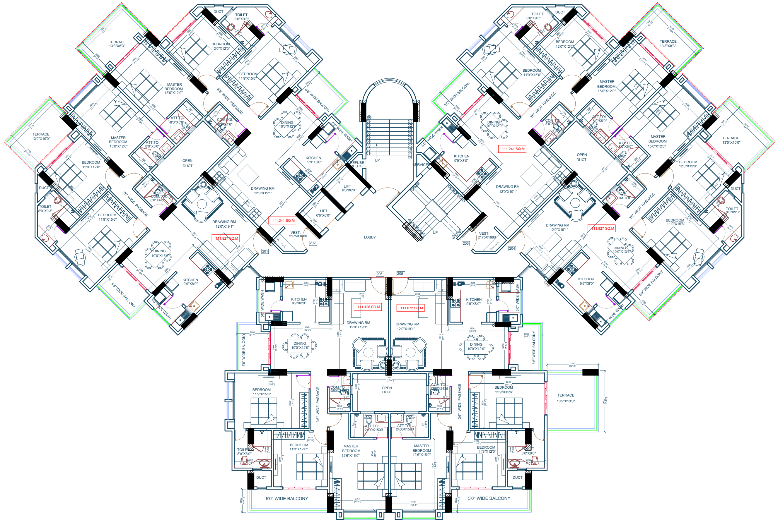
TYPICAL EVEN FLOOR PLAN
