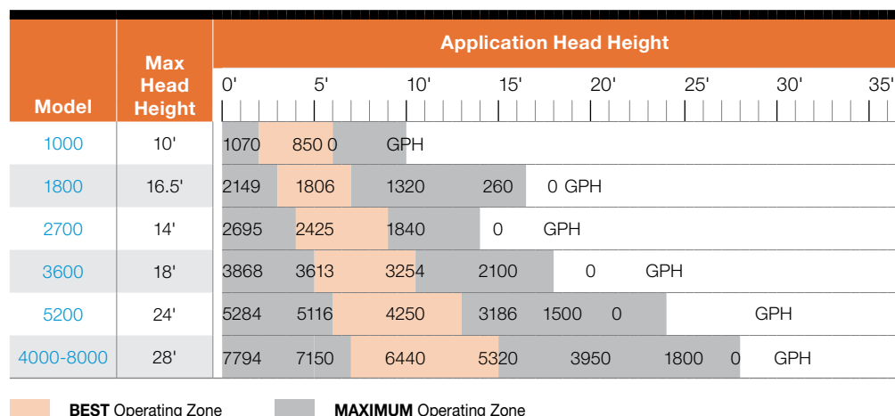
AquaForce Pond Pump Flow Chart (GPH)
