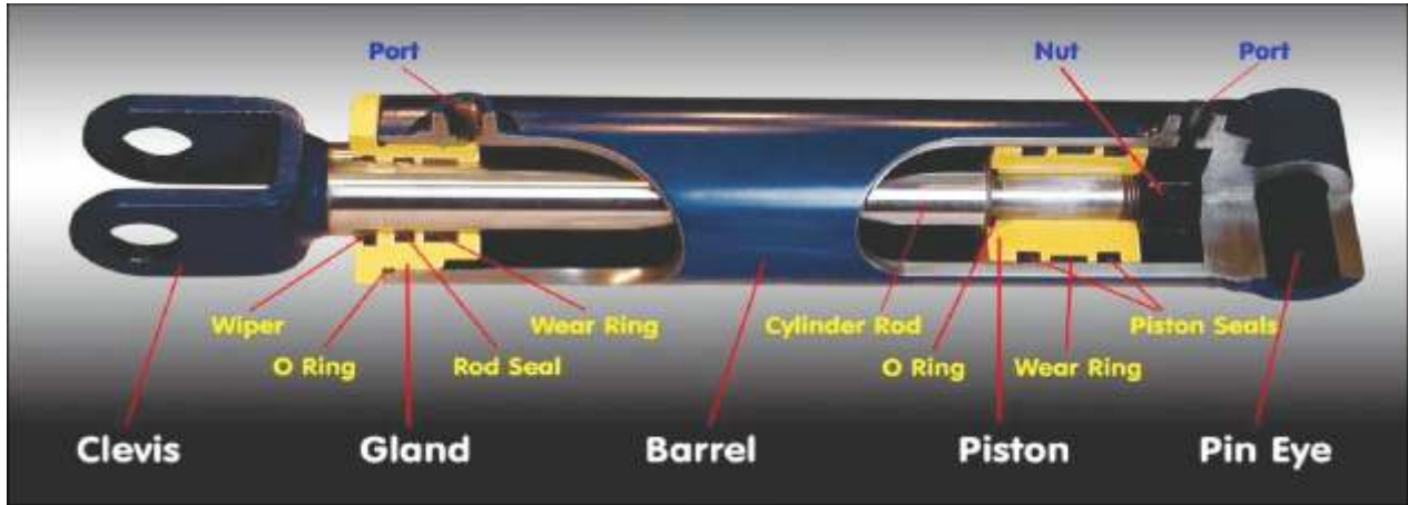
Hydraulic Cylinders
