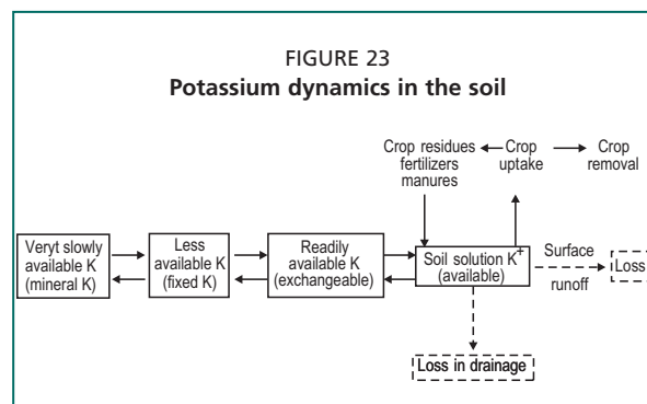
Potassium dynamics in the soil Source: After A. E. Johnston (www. Kemira-growthow.com).
