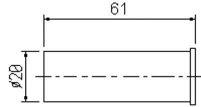
S8/031P Pin WT36.6
