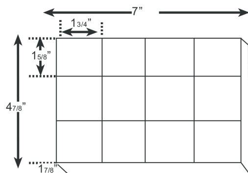
Part No. BX12
