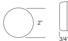
Part No. MZ-146 Marker and Clearance Grommet Mount
