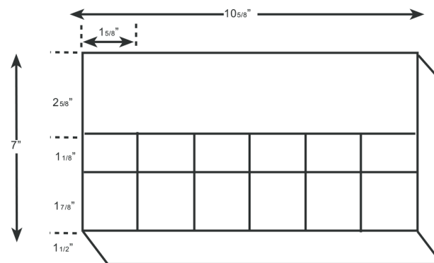
Part No. BX13
