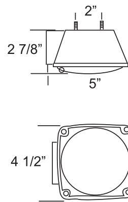
Part No. MZ-440L Turn, Tail, Stop, License Illuminator Bolt-on
