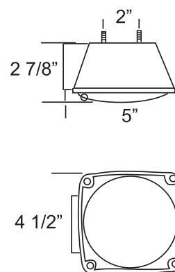
Part No. MZ-440 Turn, Tail and Stop Bolt-on
