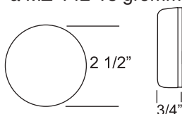
Part No. MZ-143 Marker and Clearance Grommet Mount
