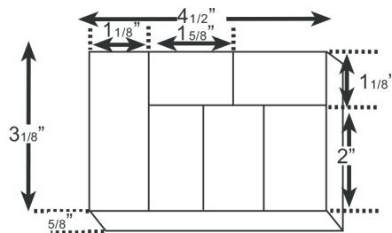
Part No. BX06
