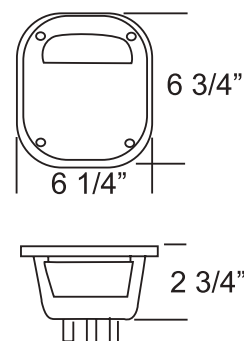
Part No. MZ-445 Turn, Tail, Stop and Backup Bolt-on
