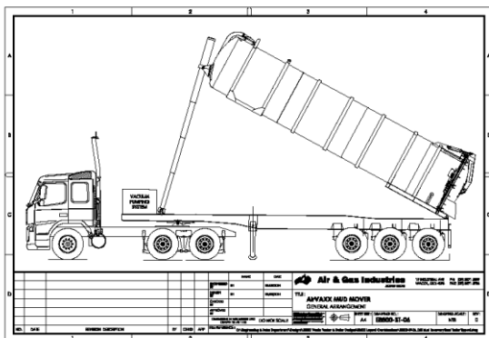
AirVAXX Mud Mover and Vacuum Trailer
