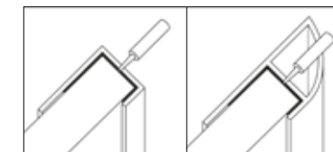
Finishing end trims and Quadrant trims Finishing end trims for panels.
