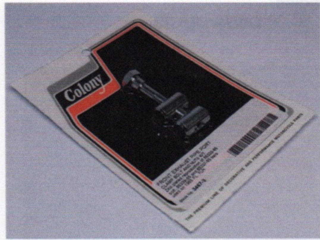
Part No. 3467-3 FRONT EXHAUST PIPE PORT CLAMP BOLT AND NUTS KIT Zinc plated reproduction of 65332-65 bolt, 65339-65 and 65337-65 bars used on 1965 FL, FLH. Retail: $20.00 Dealer: $13.00
