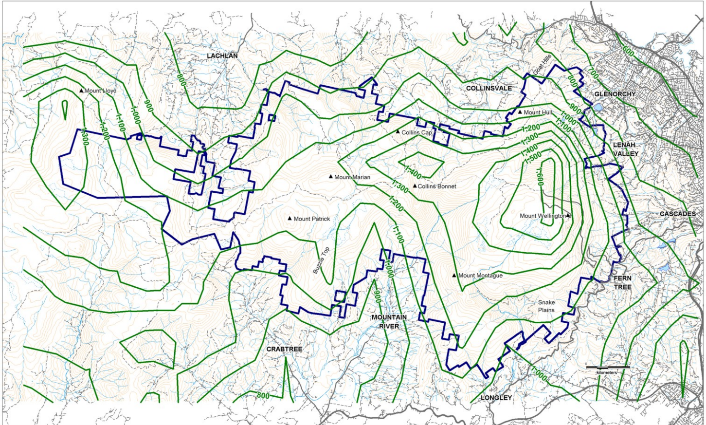
FIGURE 2 - Mean Annual Rainfall in Wellington Park
