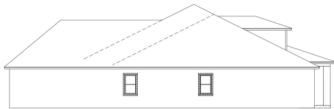
RIGHT VIEW
