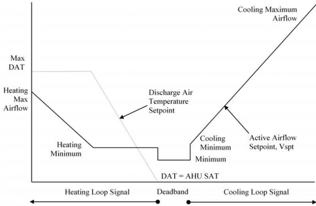
Control logic for VAV reheat zone
