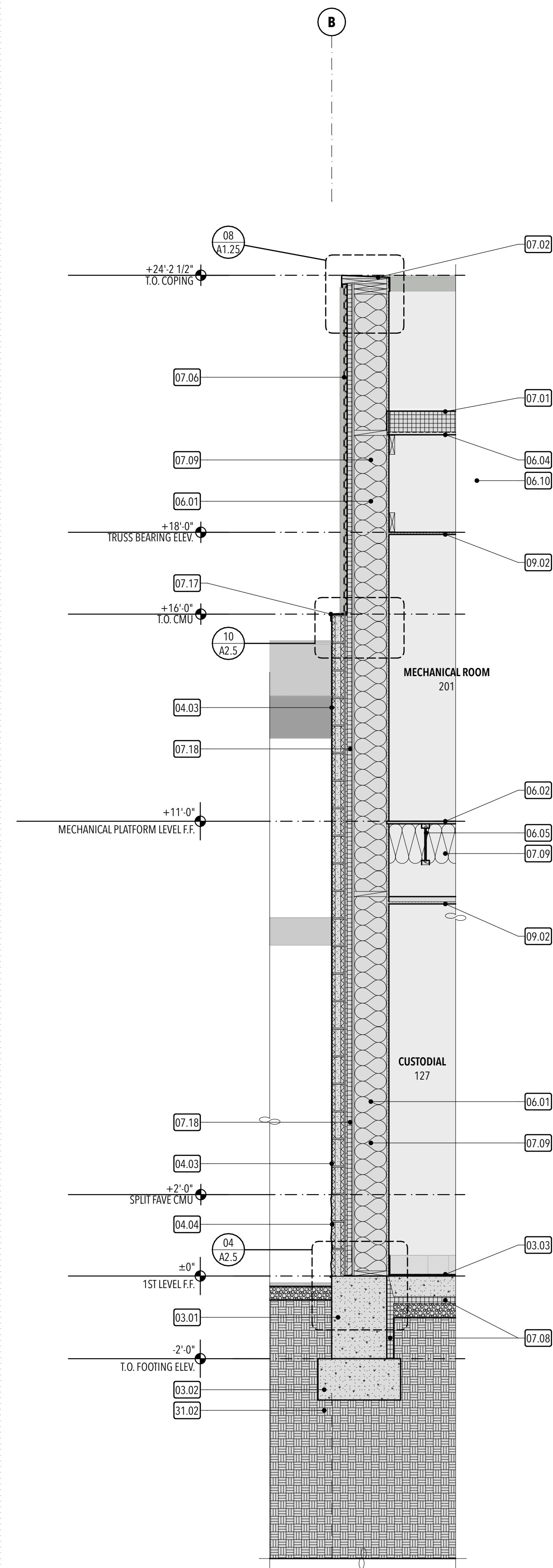
WALL SECTION 13
