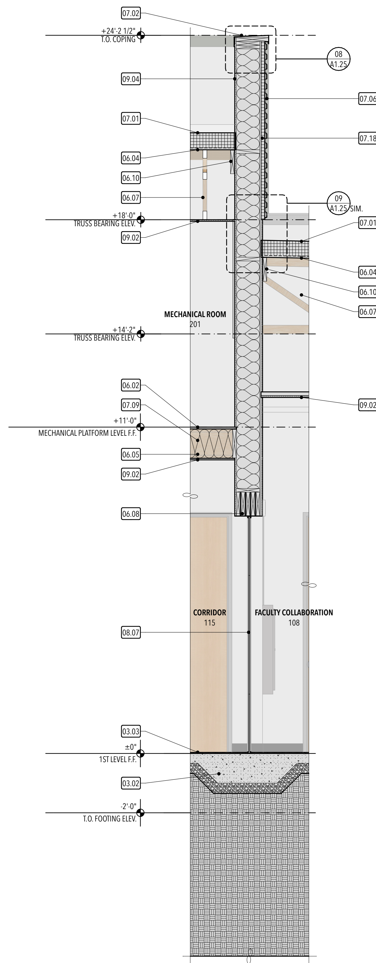
WALL SECTION 14
