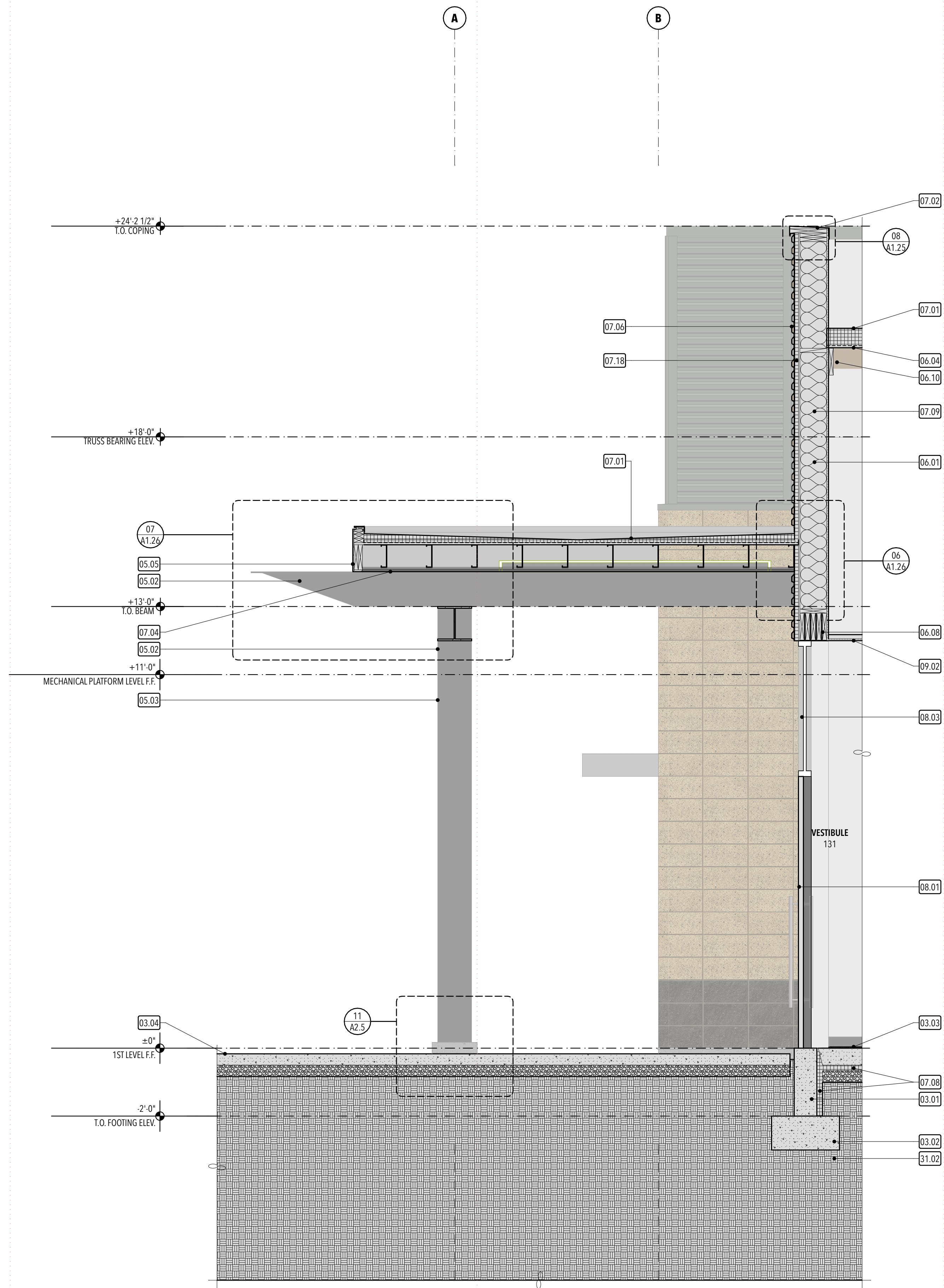
WALL SECTION 15
