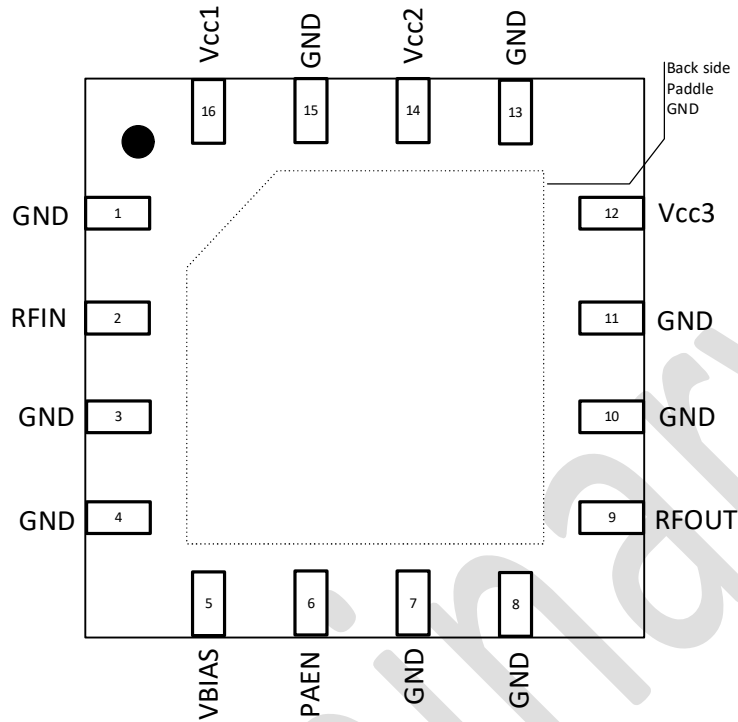
Figure 2 SP6487 Pin Diagram (Top View)
