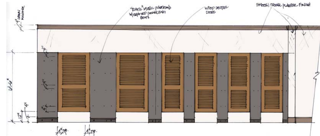
ELEVATION @ RESTROOM STALLS
