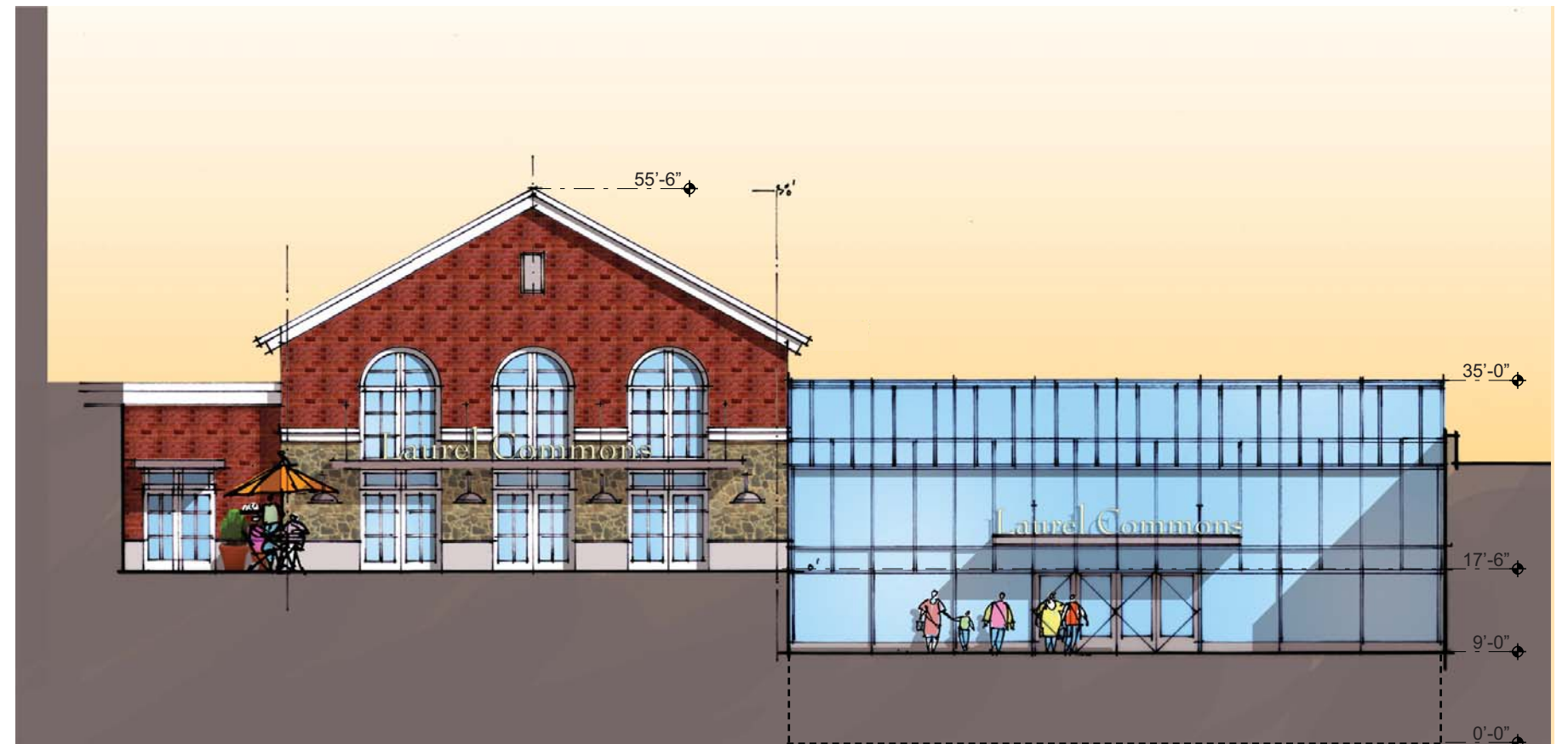
A FOOD COURT ELEVATION WEST PLAZA ENTRY
