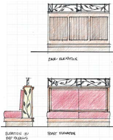
ELEVATIONS @ TYPICAL BANQUETTE
