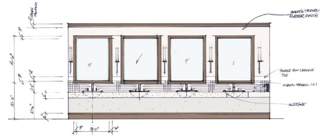
ELEVATION @ RESTROOM LAVATORY COUNTER
