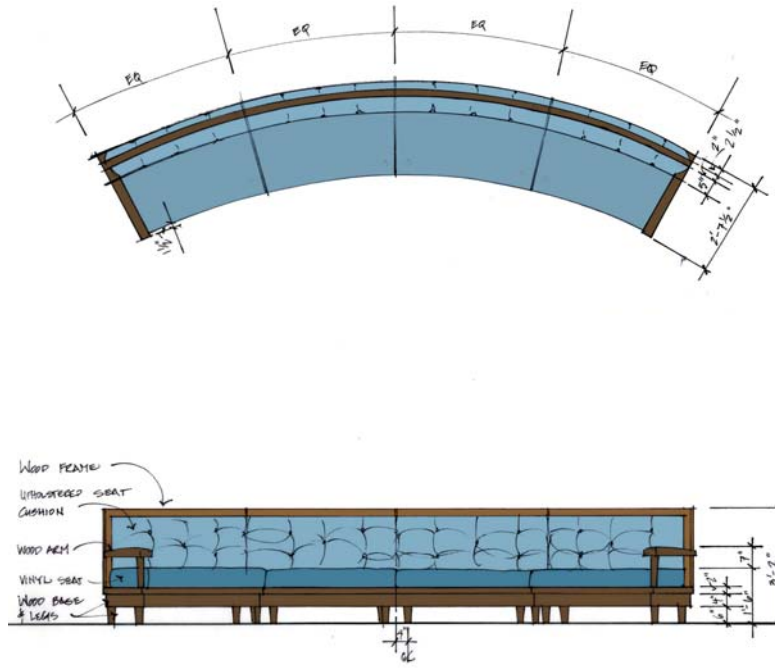
PLAN / ELEVATION @ TYPICAL CURVED BANQUETTE
