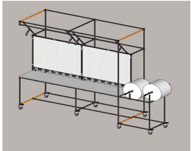
Packaging Station 2
