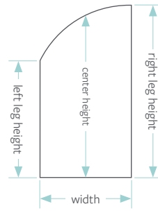
HALF ARCH LEFT
