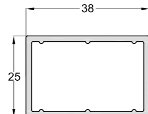
Traverso intermedio spalla Intermediate Horizontal Profile P10501
