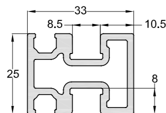
Profilo Posteriore Spalla Back Profile P10502
