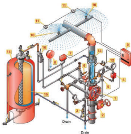
DELUGE WATER SYSTEM
