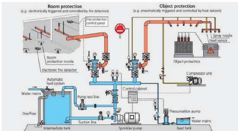
DELUGE WATER SYSTEM
