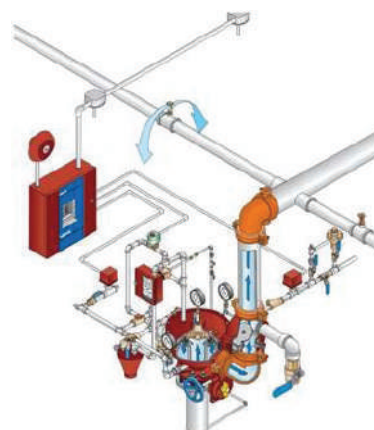
PRE-ACTION SYSTEM
