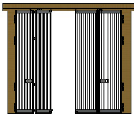
INTERIOR VIEW - DOORS PARTIALLY OPEN
