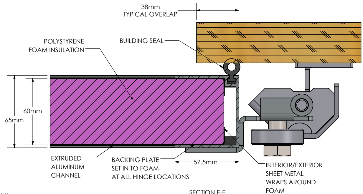
SECTION E-E
