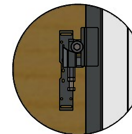
DETAIL C TYPICAL NON-LIFTING HINGE
