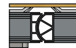
DOOR SEAL DETAIL
