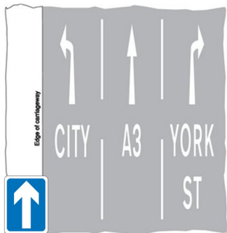
Indication of traffic lanes
