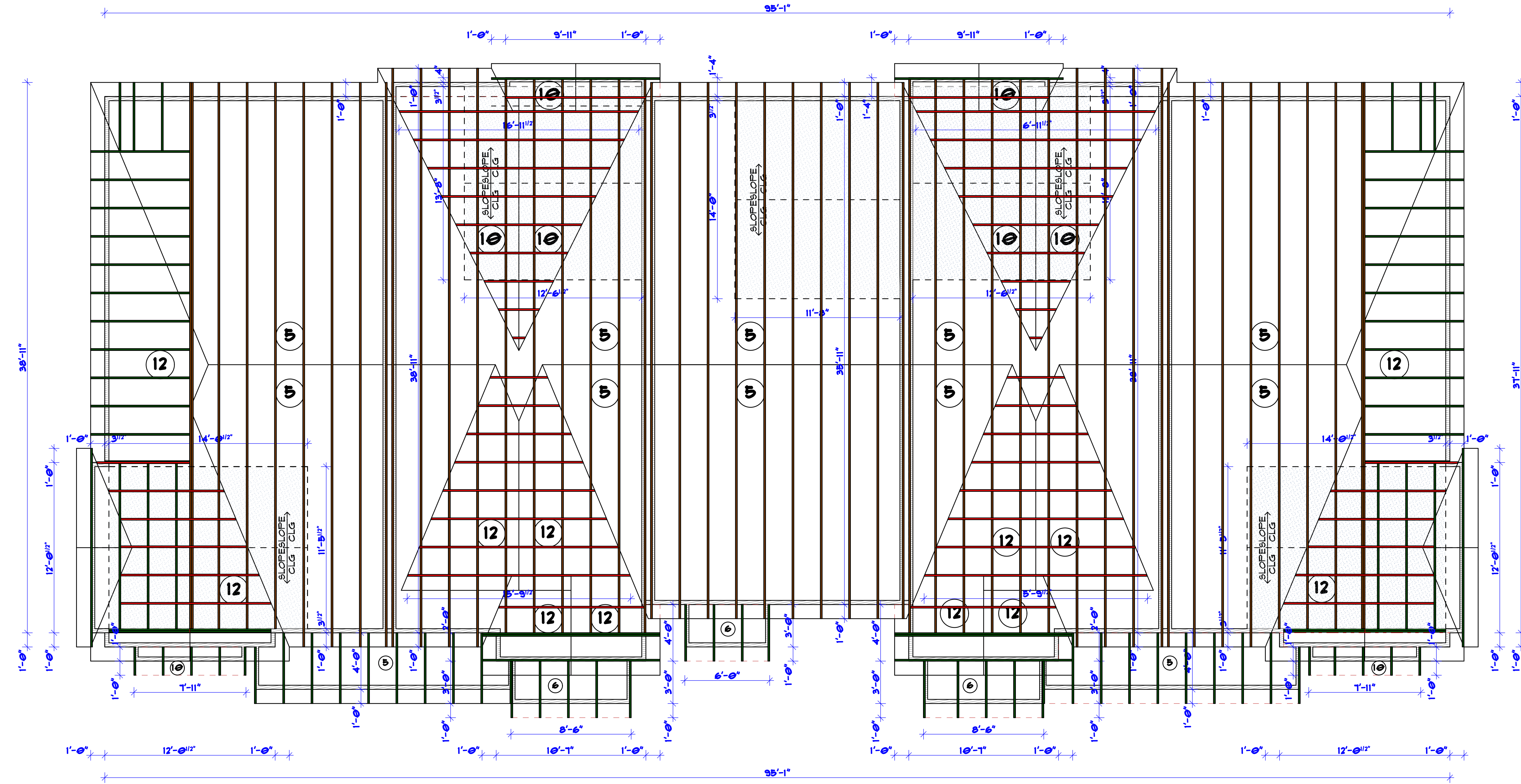
ROOF LAYOUT SCALE 1/4" = 1 FOOT
