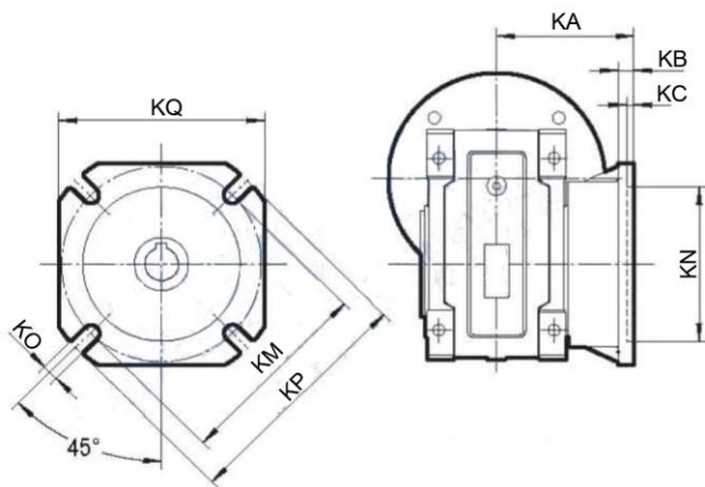
Output Flange
