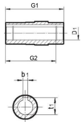
Output Hub
