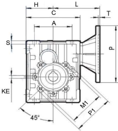
Output Flange
