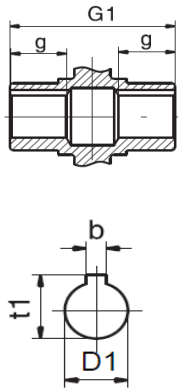
Output Hub
