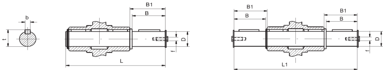
Output shafts
