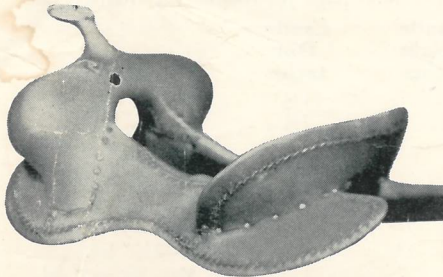
No. 155—LOW DOWN BRONC Fork swell, 14"; fork height, 8½"; cantle height, 3"; cantle dish, 1½".
