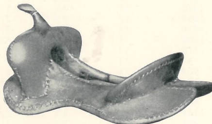
No. 574—LITTLE WONDER Fork swell, 13"; fork height, 8¼"; cantle height, 3"; cantle dish, 1¼".
