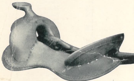
No. 391—ROCKY MOUNTAIN ROPER Fork swell, 13"; fork height, 8½"; cantle height, 3"; cantle dish, 1". No. 22—Mexican horn extra.
