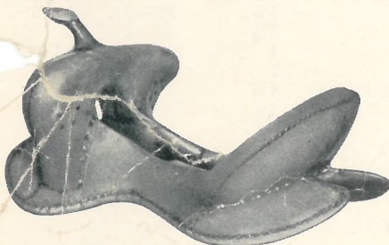
No. 1418—HEISER MASTER FITS 'EM Fork swell, 15"; fork height, 9¼"; cantle height, 5"; cantle dish, 1¾".
