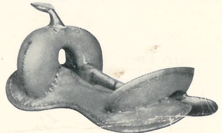
No. 1932—CURTIS ROPER Fork swell, 13"; fork height, 8½"; cantle height, 2½"; cantle dish, 1". No. 15—Mexican nickel horn extra.
