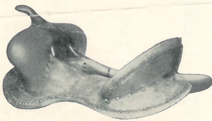
No. 794—SID SPECIAL Fork swell, 14"; fork height, 8½"; cantle height, 3½"; cantle dish, 1½".
