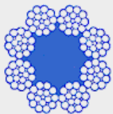
8x21 Filler Fiber Core
