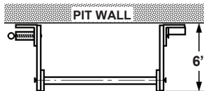
TOP VIEW - LADDER UNFOLDED
