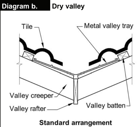
Figure 3.5.1.2 TILED ROOF FLASHING AND OTHER DETAILS
