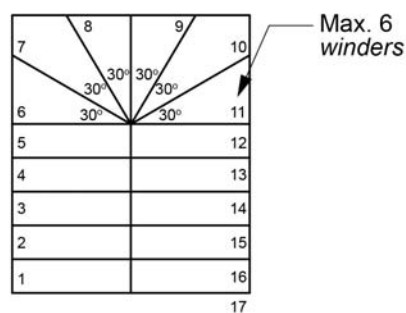
(d) Continuous stairway - 1 flight (180° change in direction)
