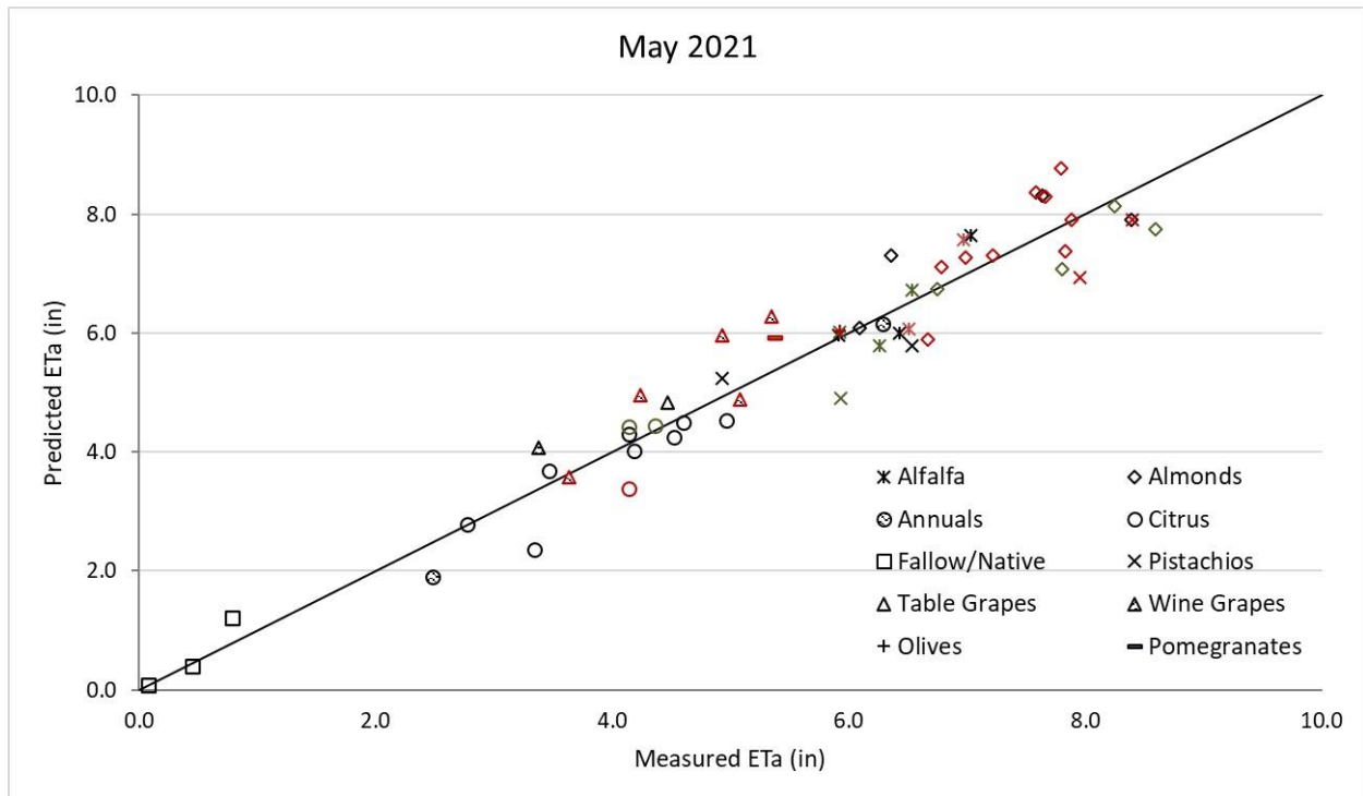
FIGURE 3. MEASURED VERSUS PREDICTED ET a FOR THE MONTH. SYMBOL COLORS REPRESENT THE STATION TYPES (BLACK = FULL, GREEN = WATER IQ (WIQ), RED = TULE TECH)
