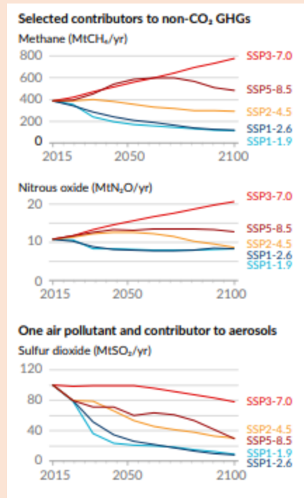
Figure 21.4 Emissions of other GHG contributors including methane and nitrous oxide and the aerosol, sulfur dioxide
