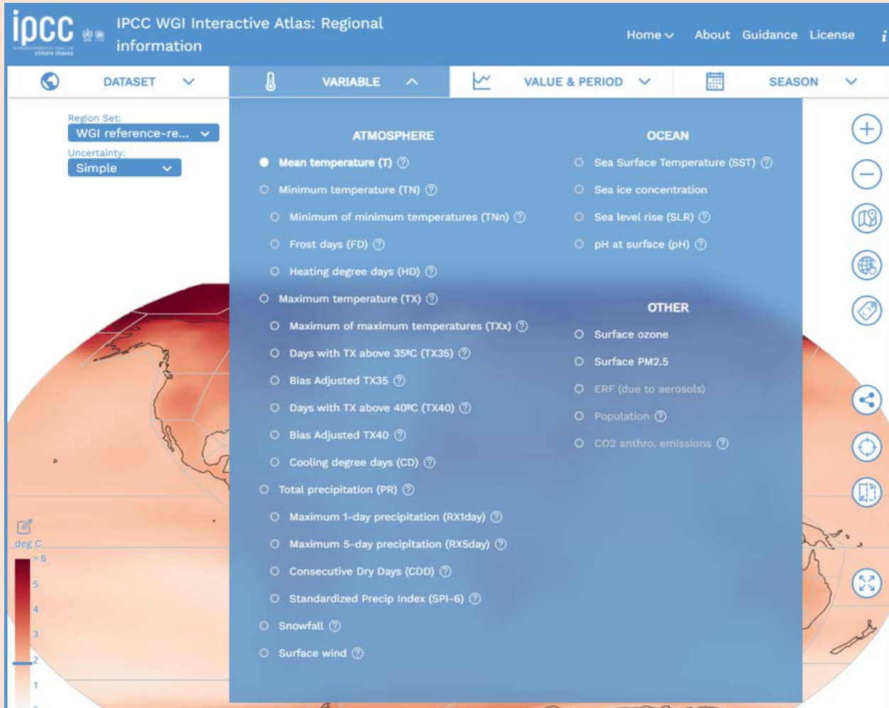
Figure 21.11 Selection of variable of interest as it relates to the atmosphere, ocean or other variables.
