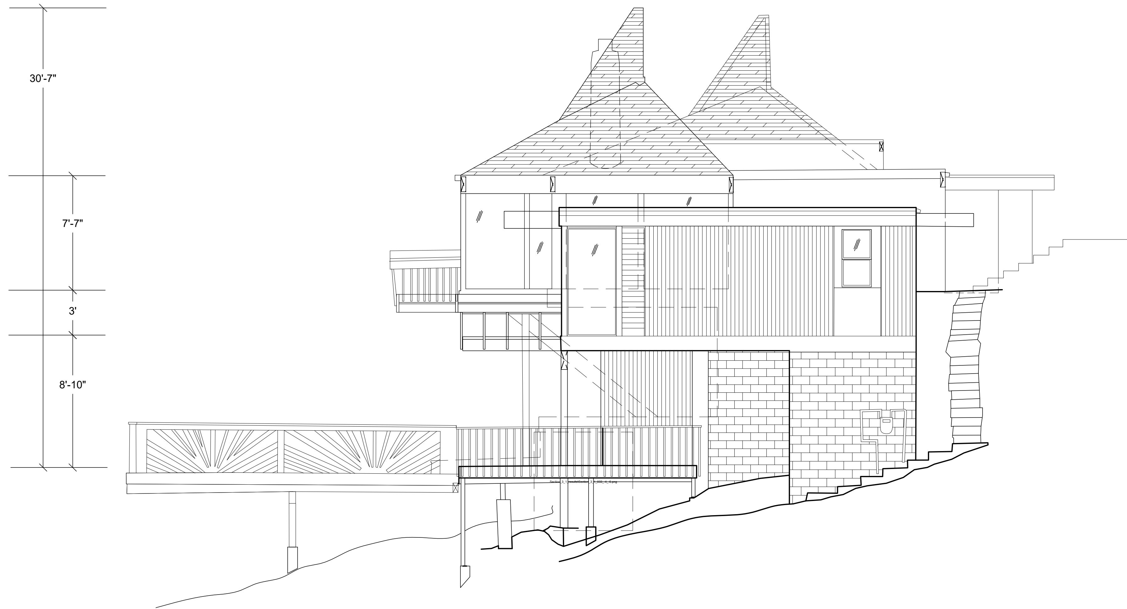
② WEST ELEVATION
