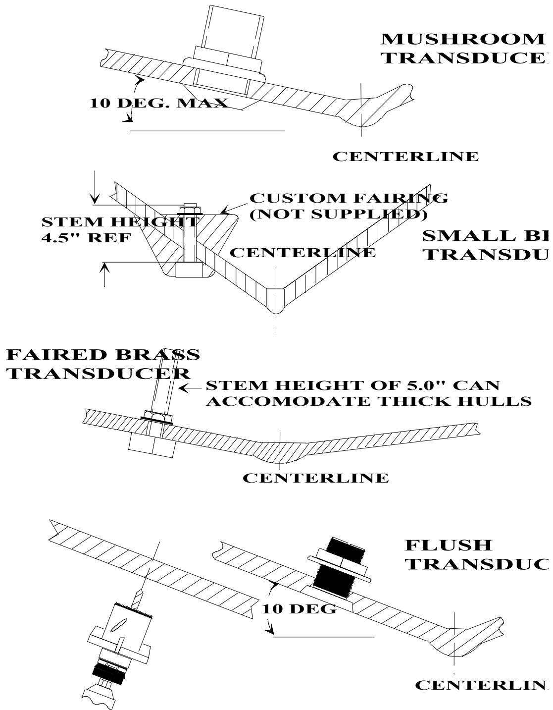
FIGURE 7.4B TRANSDUCER INSTALLATION
