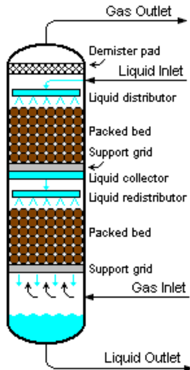
FRP ABSORBER
