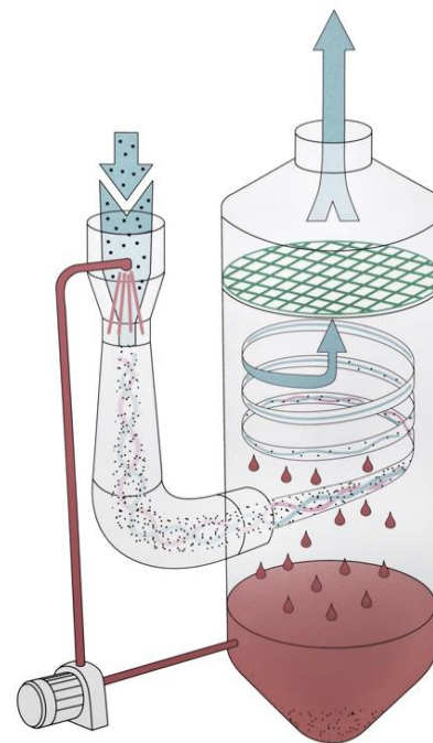
FRP VENTURI SCRUBBER
