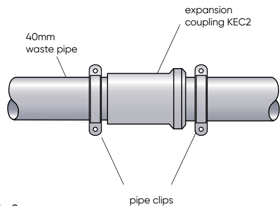
Fig 2. Ø40mm waste pipe expansion coupler. Needed where pipe length exceeds 1.8m between fixed points.
