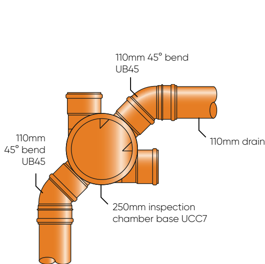
Typical 250mm inspection chamber 90° change of direction
