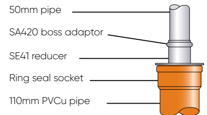
110mm PVCu to 50mm pipe
