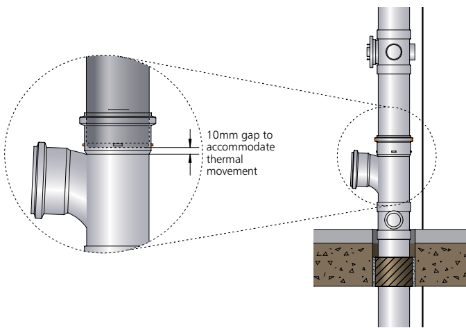
Fig 1. Typical Ø110mm soil pipe branch with push-fit ring seal joint on each floor to allow for thermal expansion
