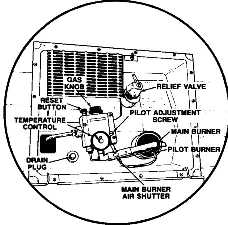
WATER HEATER (ROBERTSHAW) FIGURE 13
