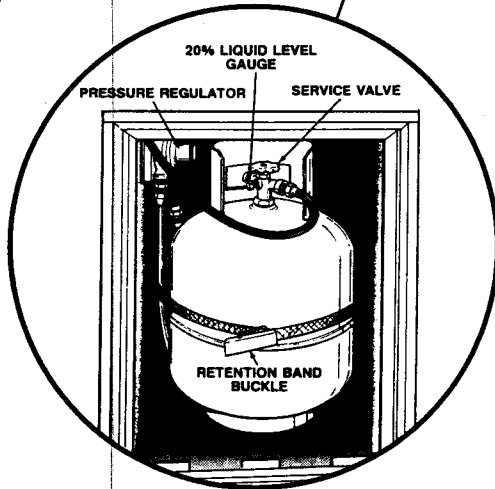
LP GAS BOTTLE FIGURE 12
