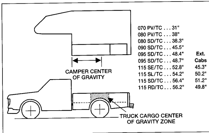
CAMPER CENTER OF GRAVITY Measured from T-wall back
