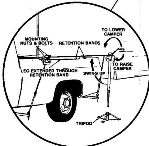
TRIPOD JACK
