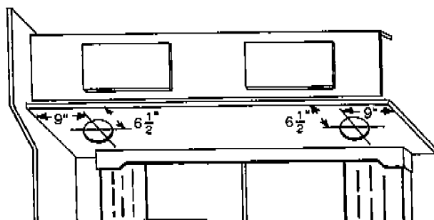
Bunk Cab - Speaker Wire Locations
