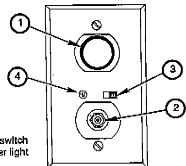
12-volt, Cable TV, Antenna Outlet
