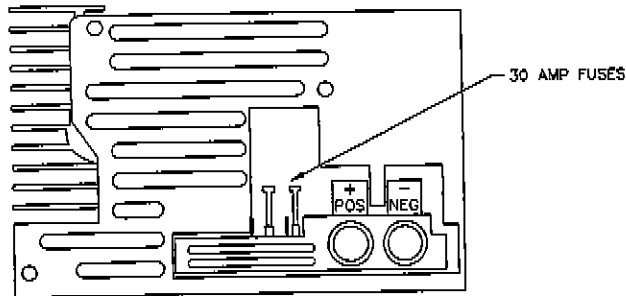
Typical Power Converter
