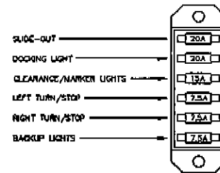
Exterior Light Fuse Box (Lance Only)
