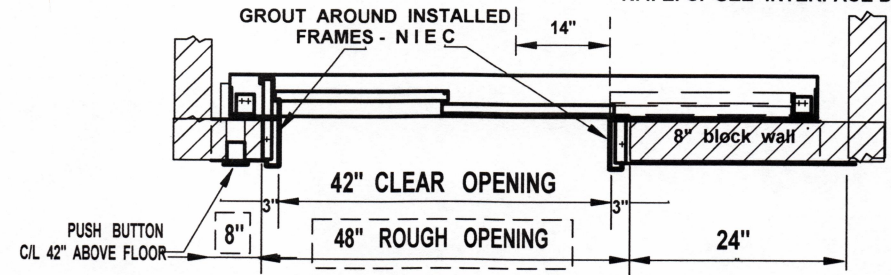
PLAN VIEW - ENTRANCES CONCRETE LEVELS
