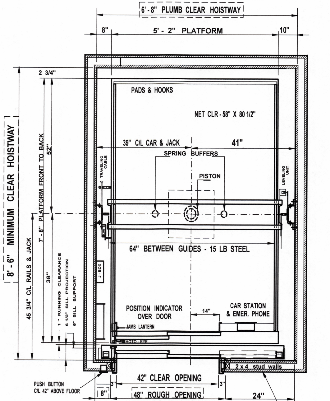
PLAN VIEW - HOISTWAY WOOD LEVELS
