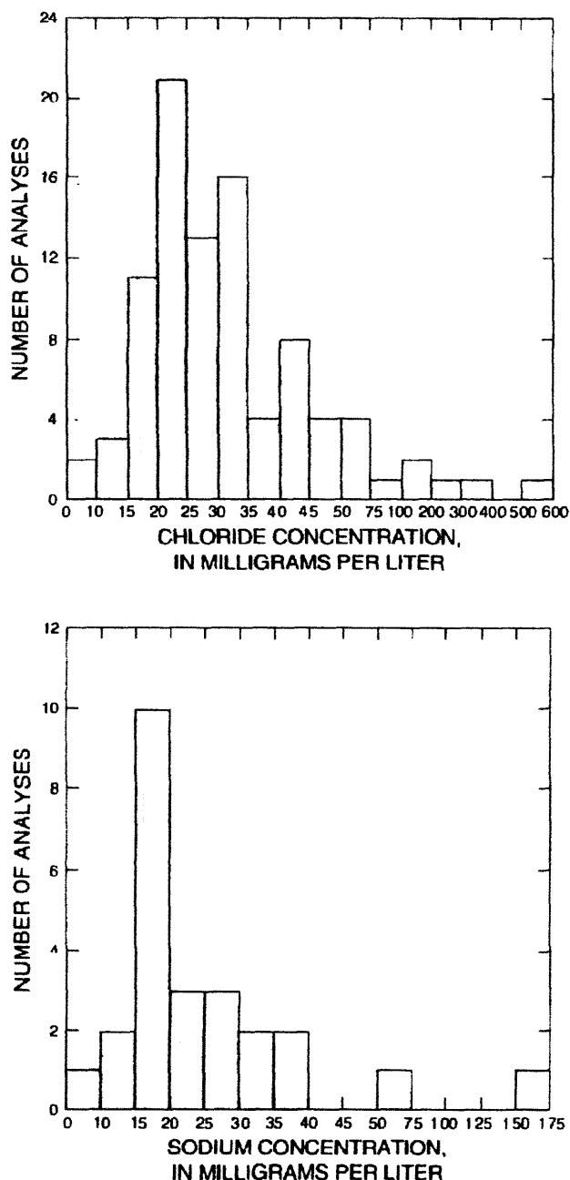
Figure 20. Frequency distributions for chloride and sodium concentrations in ground water on Block Island. (Note unequal concentration intervals.)
