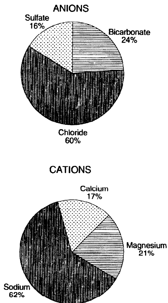
Figure 18. Average chemical composition of ground water on Block Island expressed in percentage of milliequivalents.
