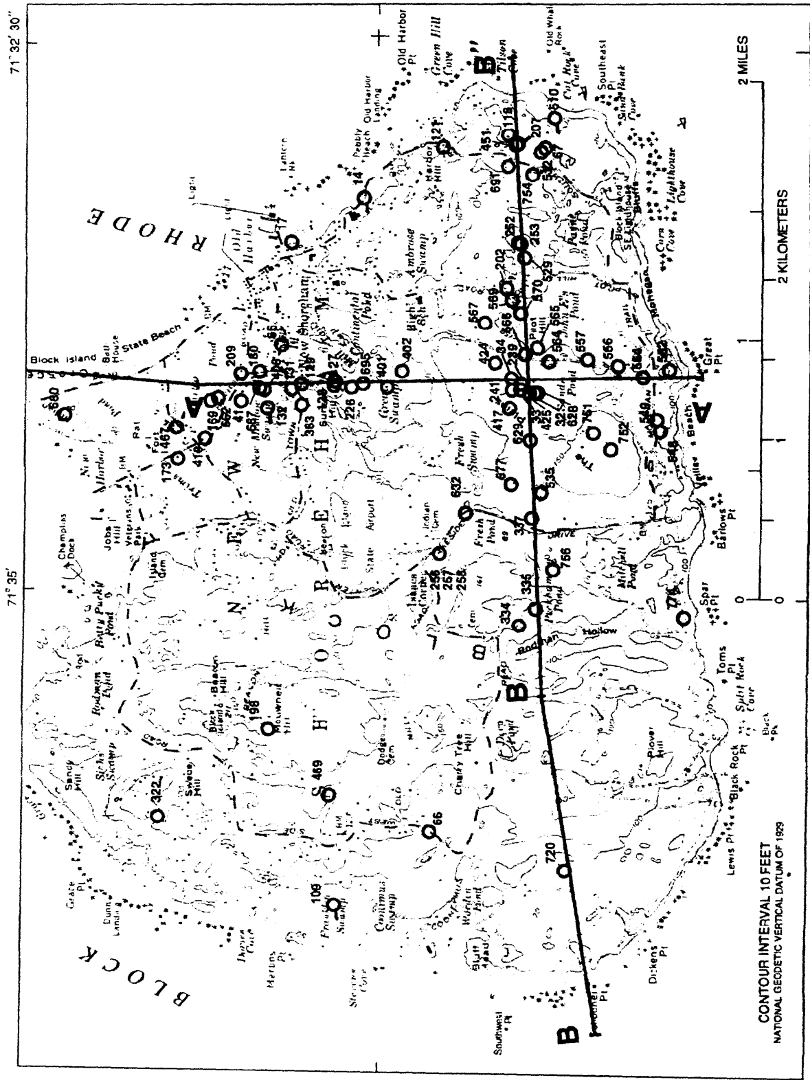
BASE FROM U.S. GEOLOGICAL SURVEY BLOCK ISLAND, 1957 PHOTO REVISSED 1970 1:24000
