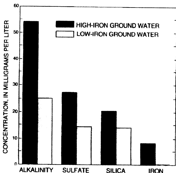
Figure 26. Average chemical compositions of high-iron and low-iron ground water on Block Island.
