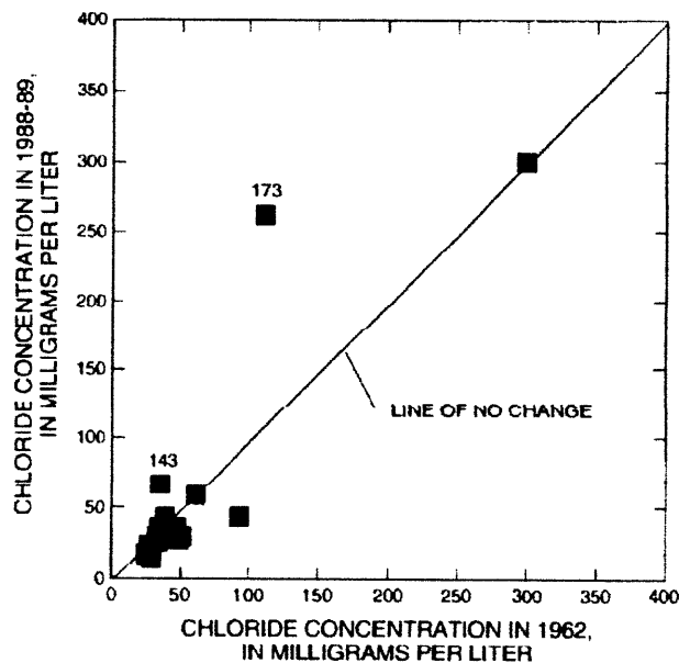
Figure 27. Change in chloride concentration in 21 wells on Block Island, 1962 and 1988-89. (Labels are well numbers.)
