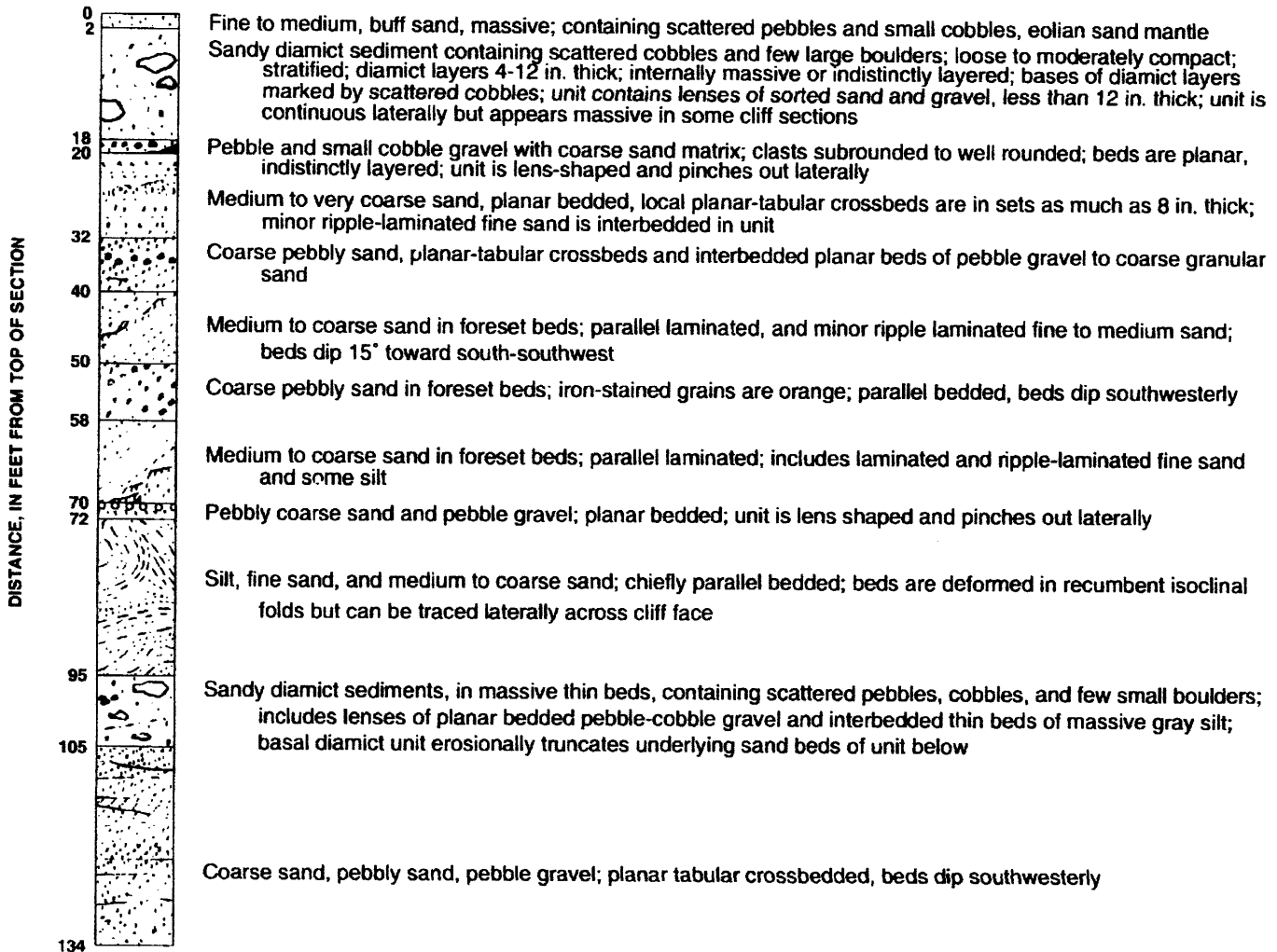
Figure 12. Measured sections of stratified diamict-sediment sequences of the upper moraine at Schooner Point and Southeast Light. (Locations of sections shown in figure 8.)
