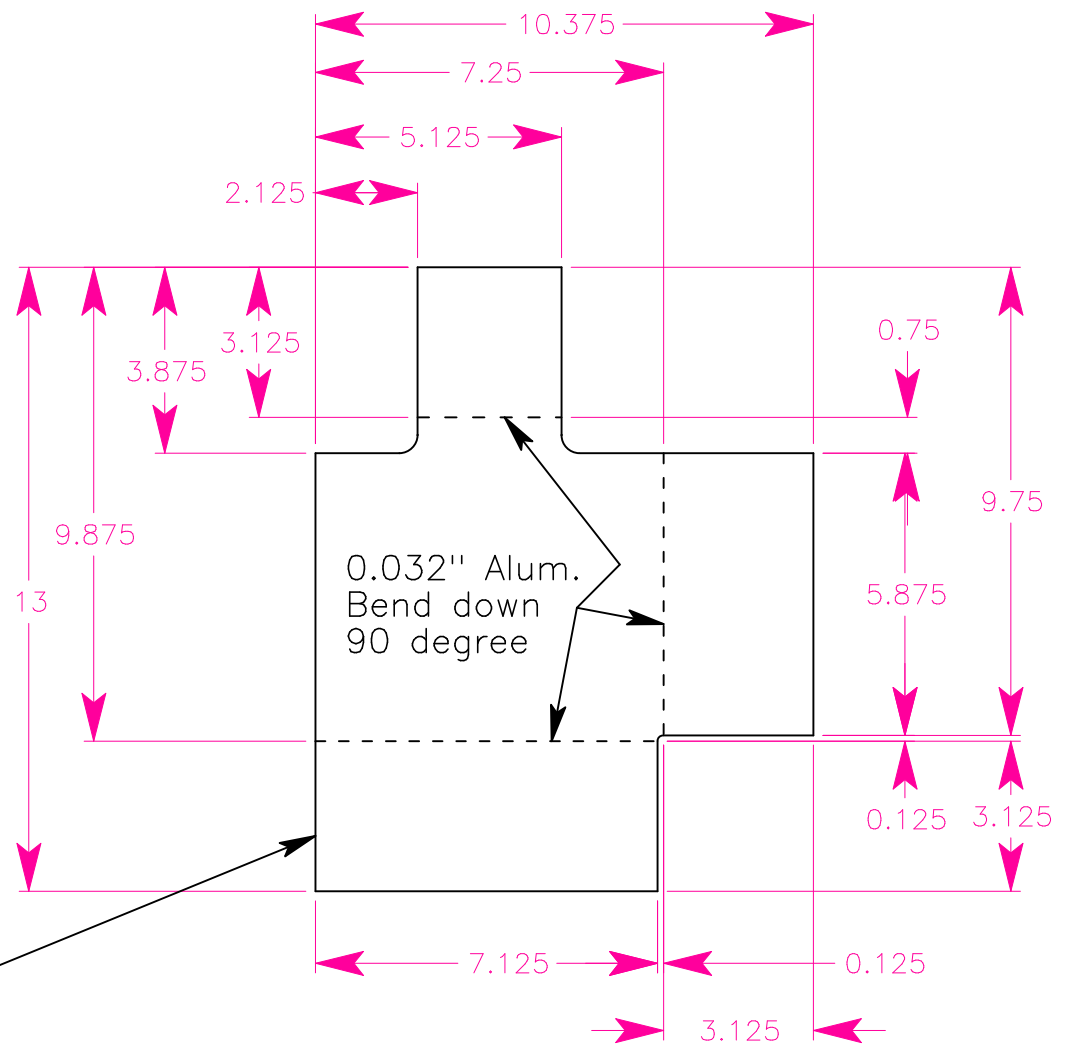
Battery Box, Flat Layout
