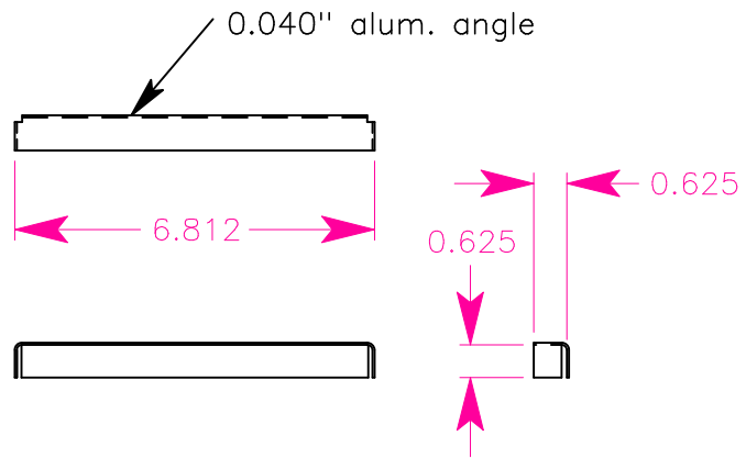
Battery Box Vert. End Angle
