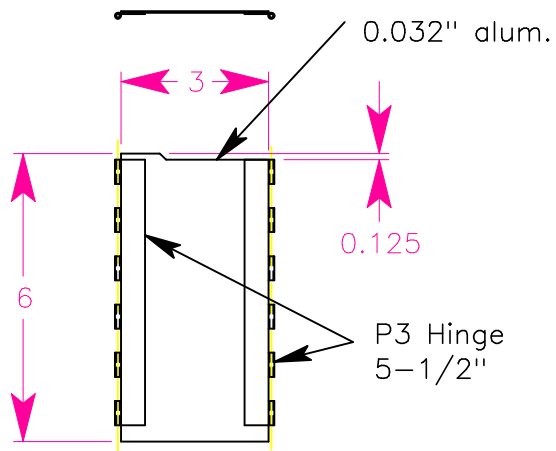
Battery Box Door
