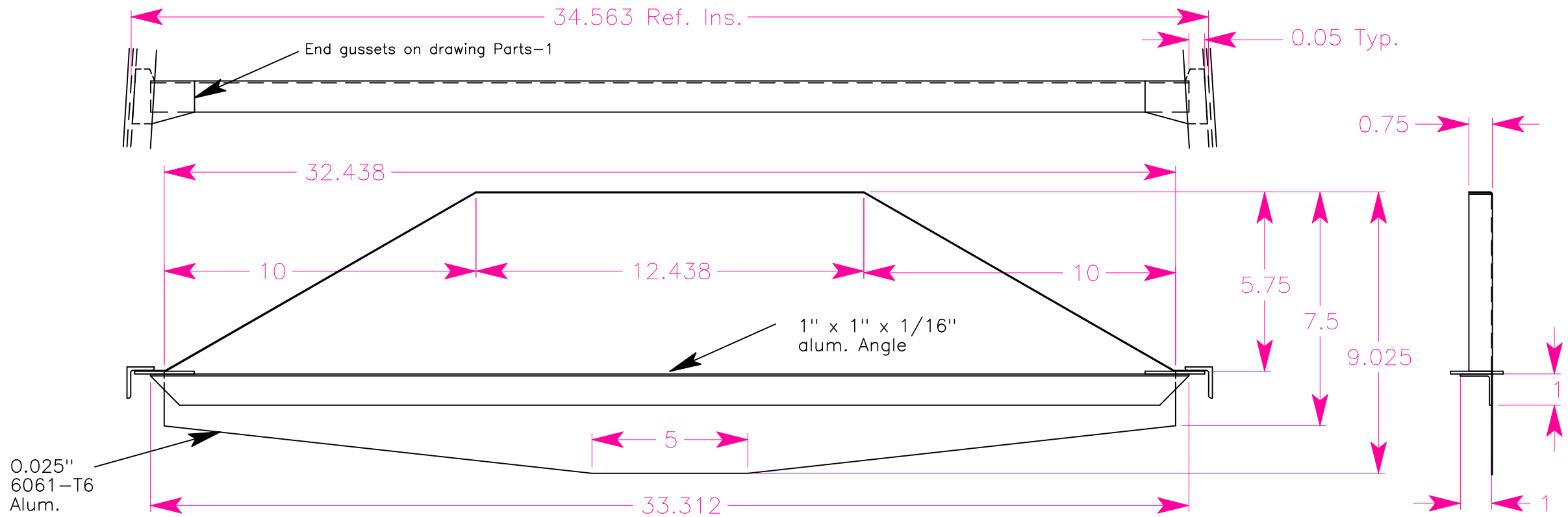
Gas Tank Shield (1)
