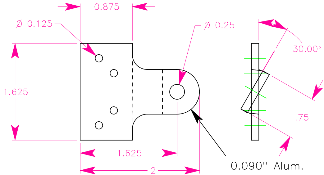
Cable Anchor, attach to vertical angle inside of firewall 1 as shown, 1 opp.
