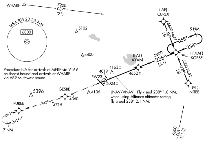
RNAV Approach
