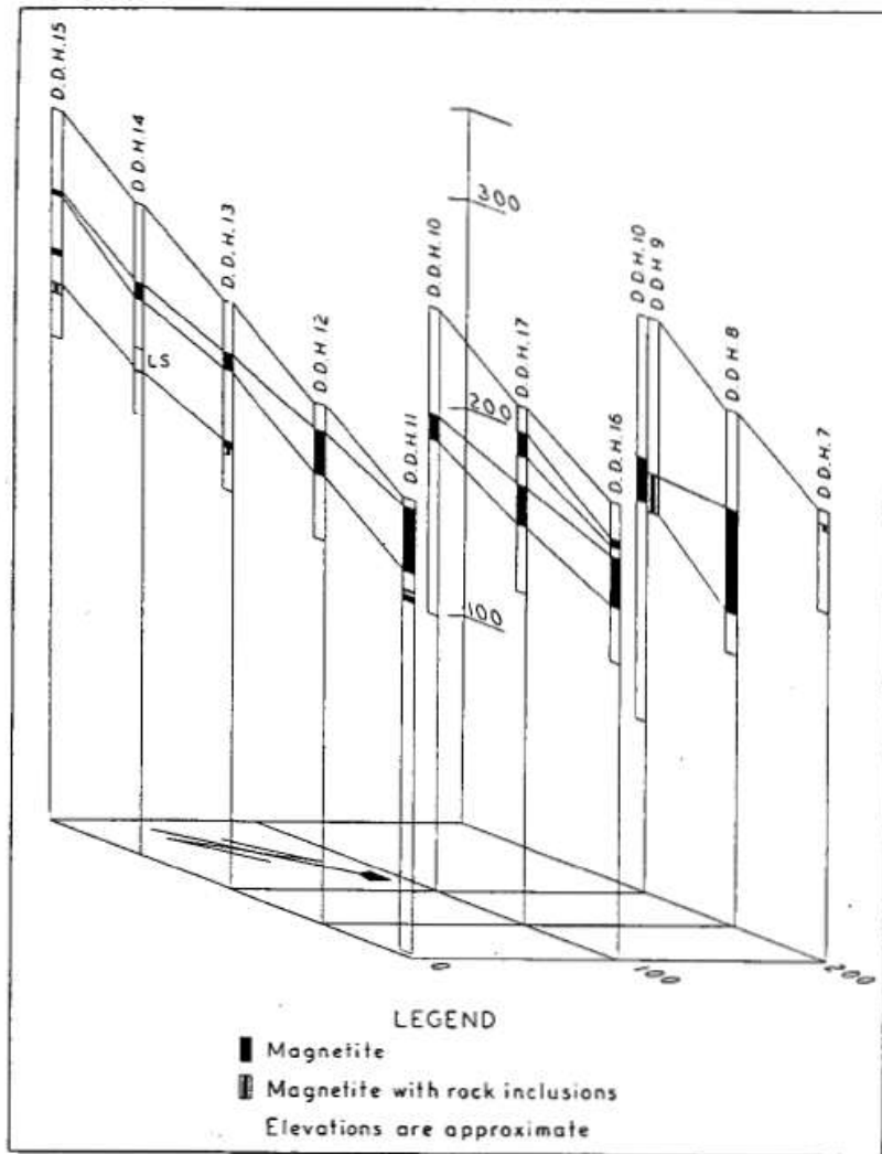
Figure 12. Diamond-drill intersections on the Iron Mike property.
