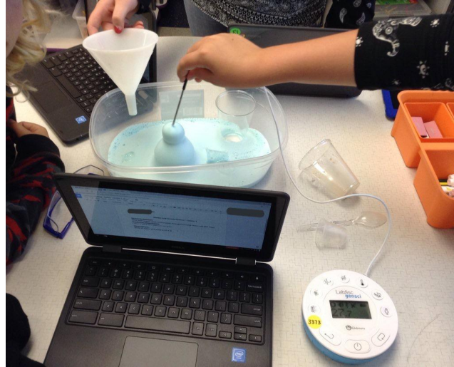
LabDisc Portable Data Collection
