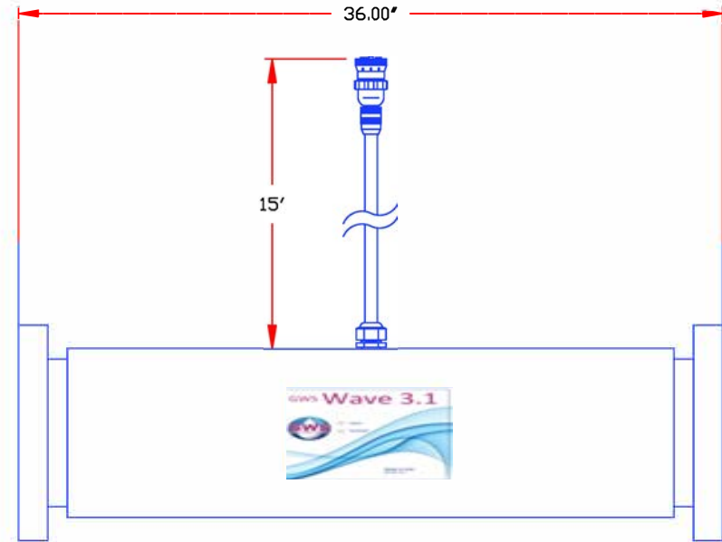
6" FLG. FRP RC ELEVATION SCH 40 PVC SHELL
