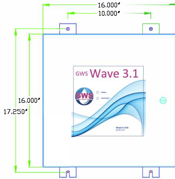
CONTROL PANEL
