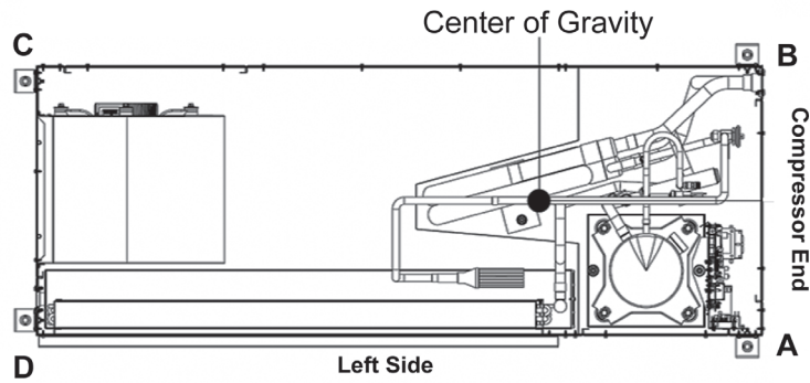
Figure 1: Horizontal Unit Corner Weights - Letter Reference for Table 4
