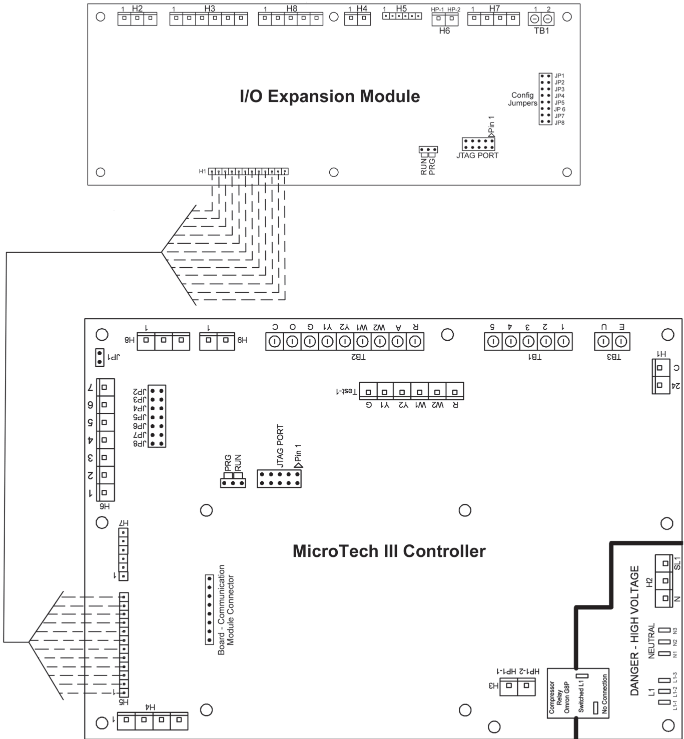
Figure 32: MicroTech SmartSource Unit Controller and I/O Expansion Module
