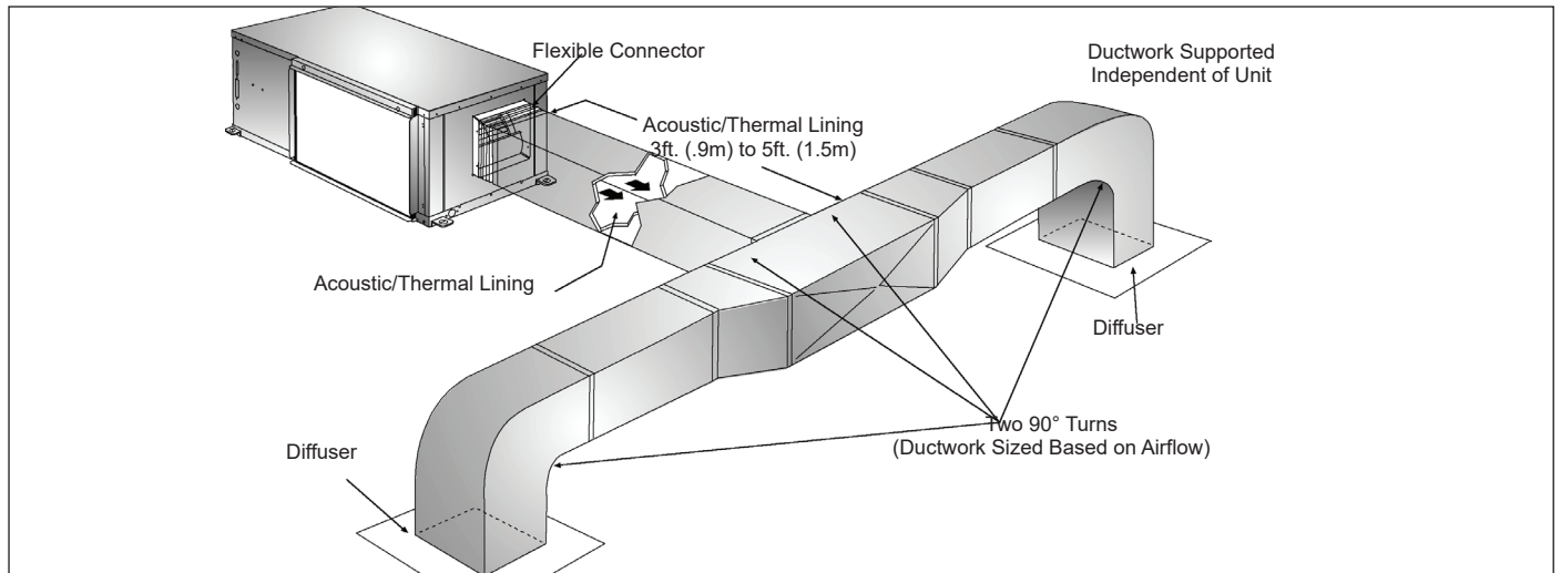
Figure 14: Typical Ducting for Horizontal Unit
