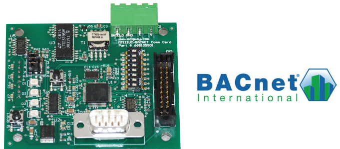
Figure 35: MicroTech III BACnet Water Source Heat Pump Snap-In Communication Module
