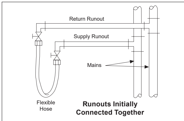
Figure 31: Supply and Return Runouts Connected Together
