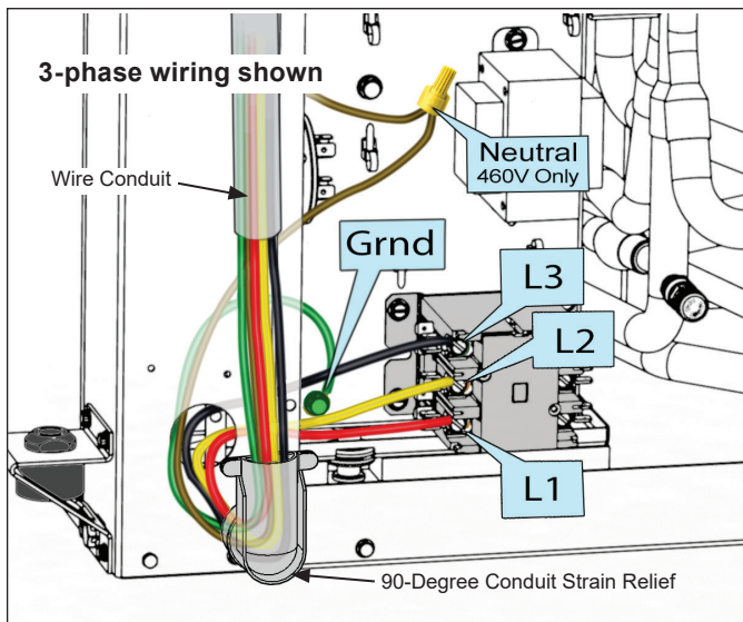
Figure 19: Route Line Voltage Wires To Terminal Screws
