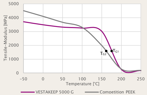
Figure 4 – Tensile Modulus between -50°C and 250°C
