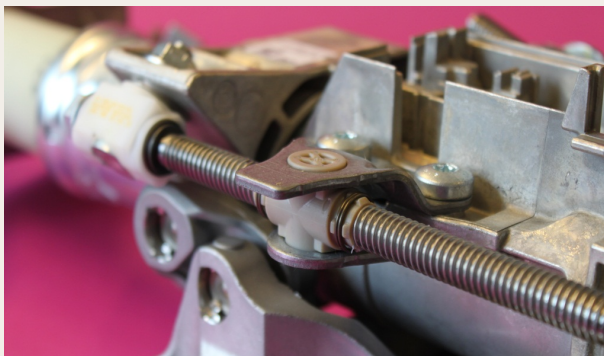
Figure 1 – Steering column adjustment assembly
