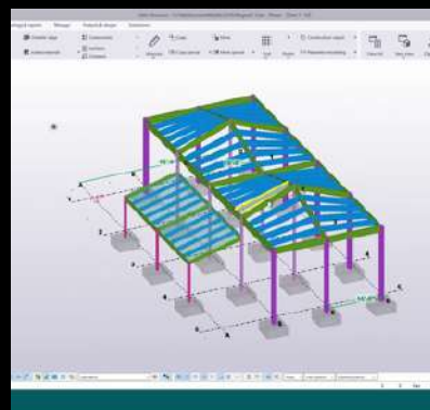
Steel Structure
